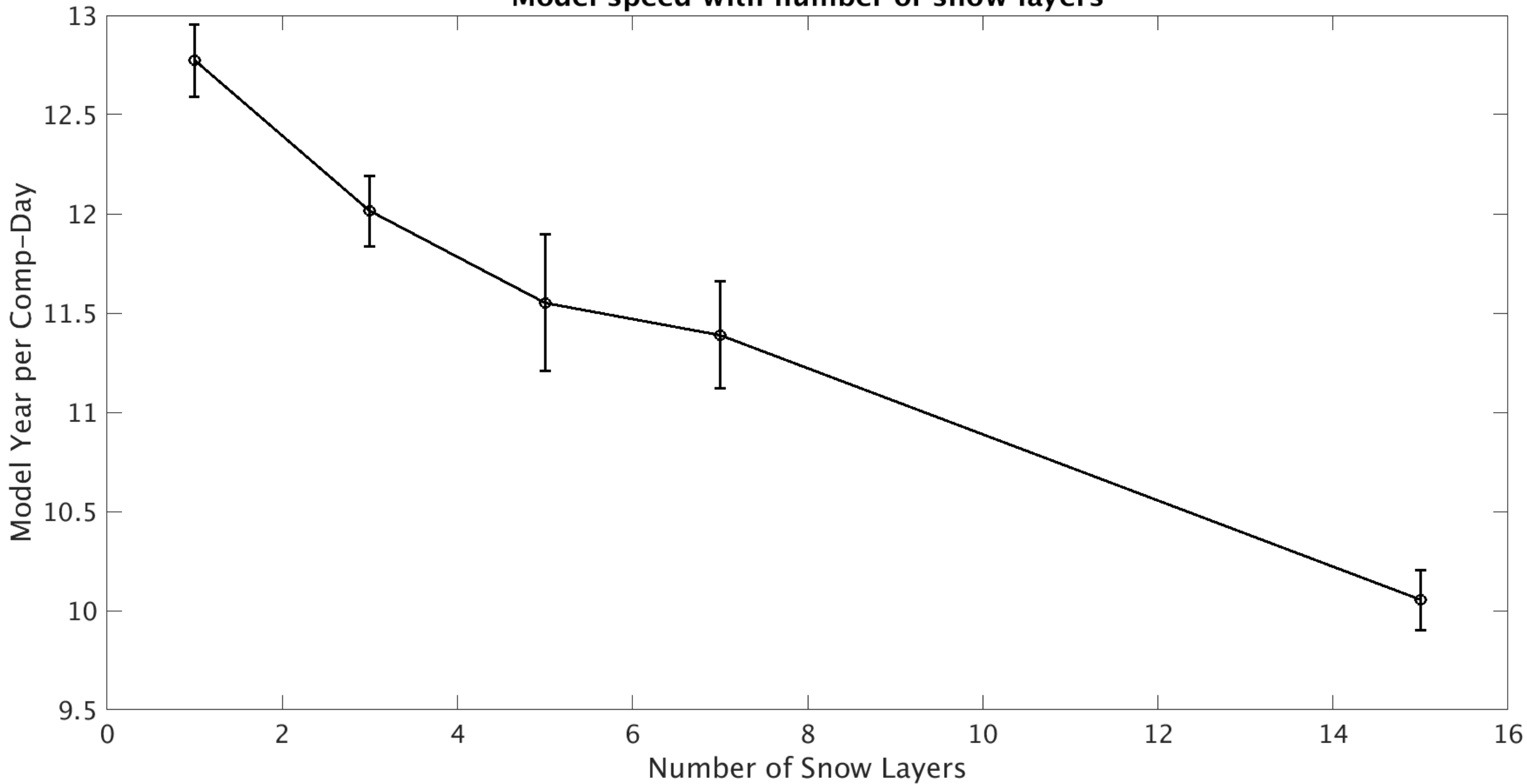
Model speed with number of snow layers
