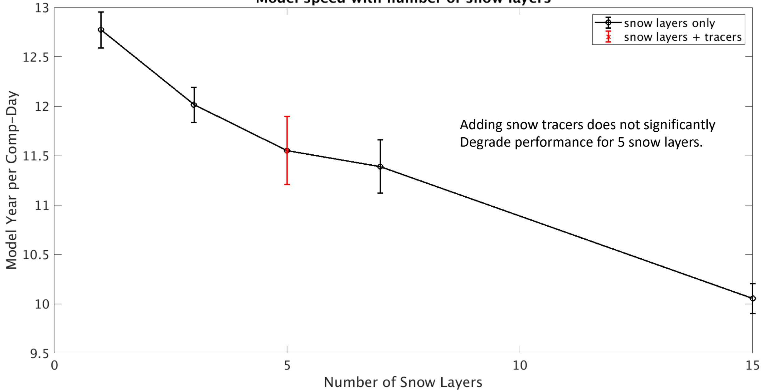
Model speed with number of snow layers
