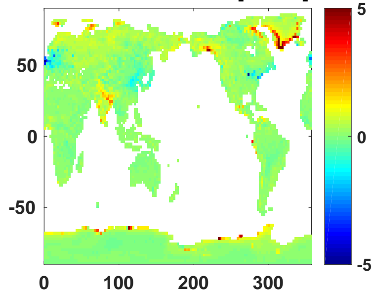
Bugfix branch
