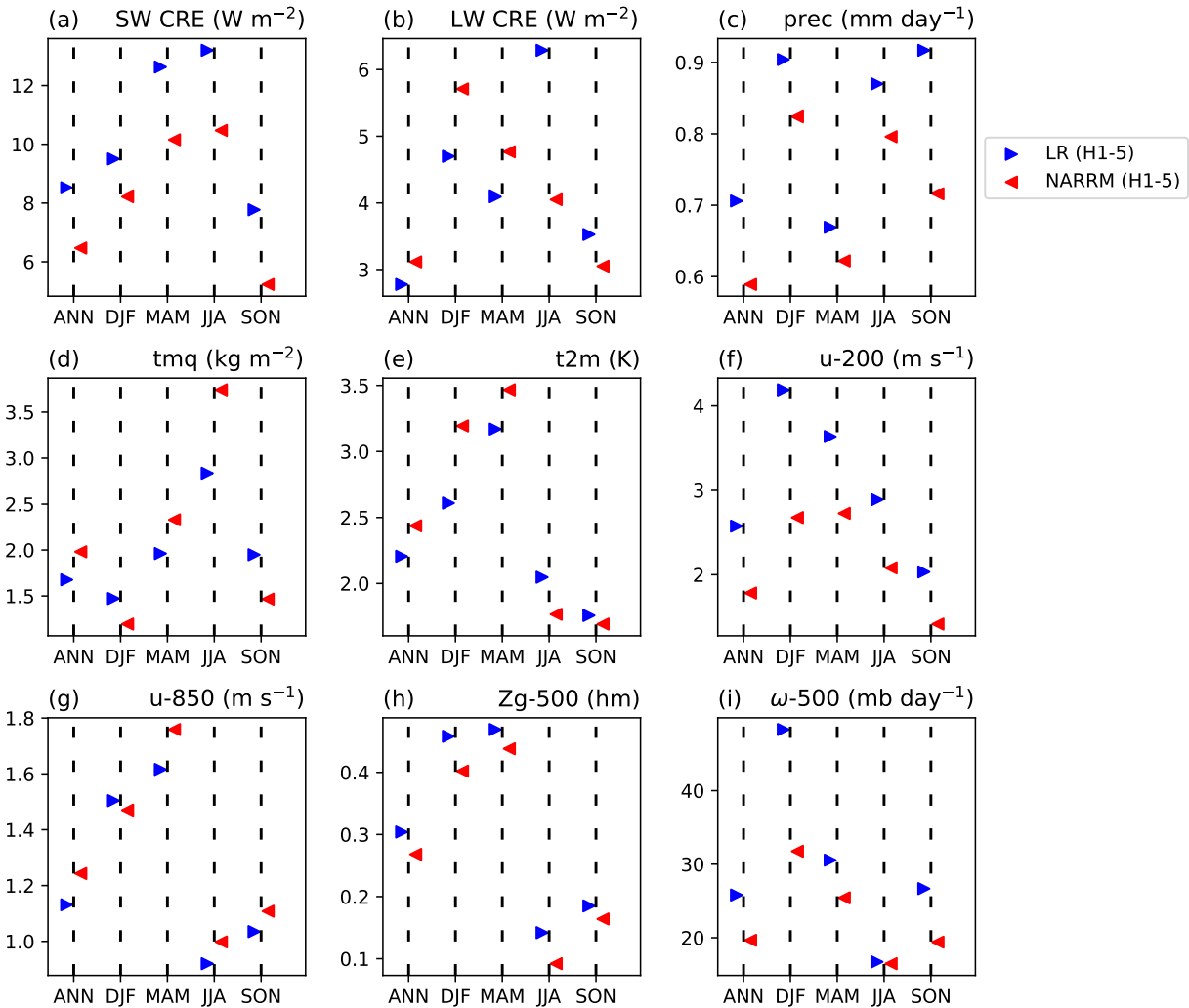
Figure 10. Same as Fig. 7, but contrasting LR and NARRM historical ensemble means at the refined CONUS area ( 20^{\circ} – 50^{\circ} N, 65^{\circ} – 125^{\circ} W). Note that variables shown are adjusted to be more appropriate for the CONUS. (a, b) TOA SW and LW cloud radiative effects, (c) precipitation, (d) total precipitable water, (e) surface air temperature, (f, g) 200- and 850-hPa zonal wind, and (h, i) 500-hPa geopotential height and vertical velocity (pressure). The same reference climatology data are used for the variables also shown in Fig. 7, whereas ERA5 (Hersbach et al., 2020) (1985-2014) for (d, e, and i).
