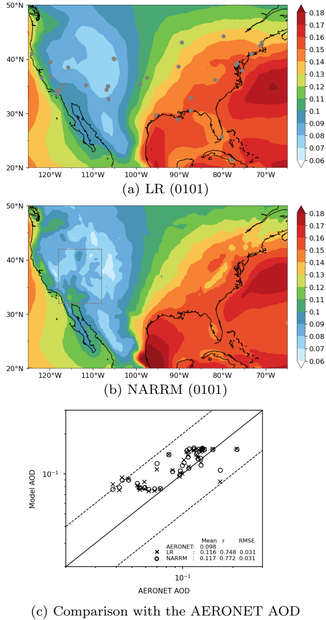
Figure 15. Aerosol optical depth (AOD) at 550 nm from (a) LR (0101) and (b) NARRM (0101) historical simulations averaged over 2000–2014. Panel (c) shows the AOD comparison of the two model simulations with the AERONET observations during 2006–2015. The site locations of AERONET are denoted by the gray dots in panel (a). The gray box in panel (b) denotes the dust region referenced in Fig. 16.
