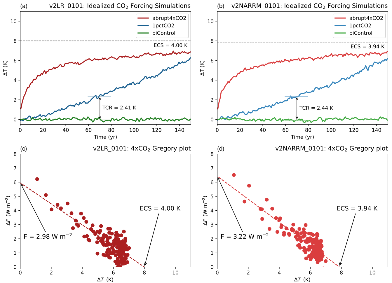
Figure 9. Comparison of climate sensitivities between LR (left) and NARRM (right) derived from idealized CO 2 forcing simulations. (a, b) time series of global annual mean surface air temperature anomaly from the following simulations, abrupt-4xCO 2 (red), 1pctCO 2 (blue), and the control ( piControl ; green). The transient climate response (TCR) is computed as a 20-year average around time of CO 2 doubling (year 70). (c, d) Gregory regression plots. The estimated effective climate sensitivity (ECS) and effective 2x CO 2 radiative forcing (F) are as labeled.
