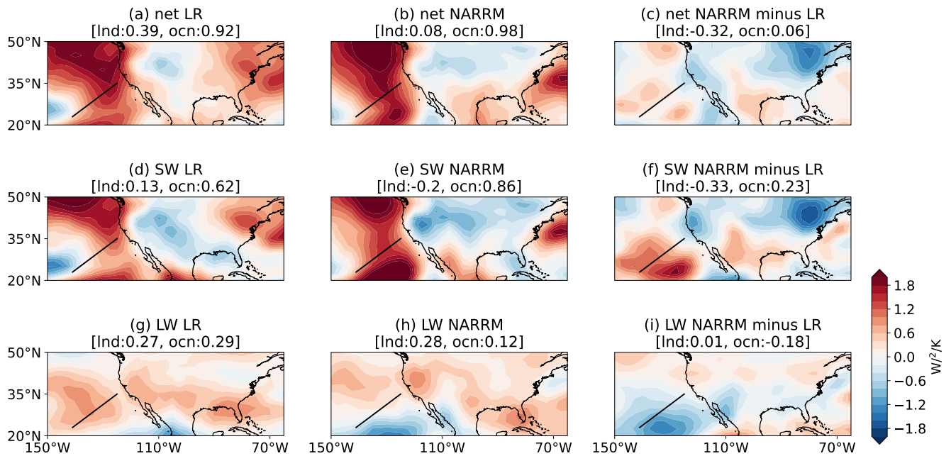
Figure 24. Spatial distribution of North America (NA) total (a-c), SW (d-f), and LW (g-i) feedbacks for LR, NARRM, and the difference between NARRM and LR. The GPCI transect (Teixeira et al., 2011) is denoted by the black line. The average values over land and ocean are labelled in the brackets.
