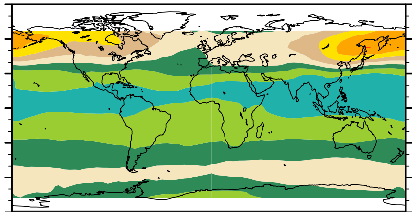
OMI/MLS satellite
