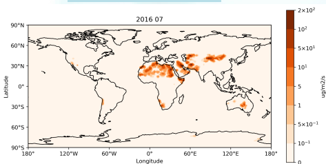
Dust Emission
