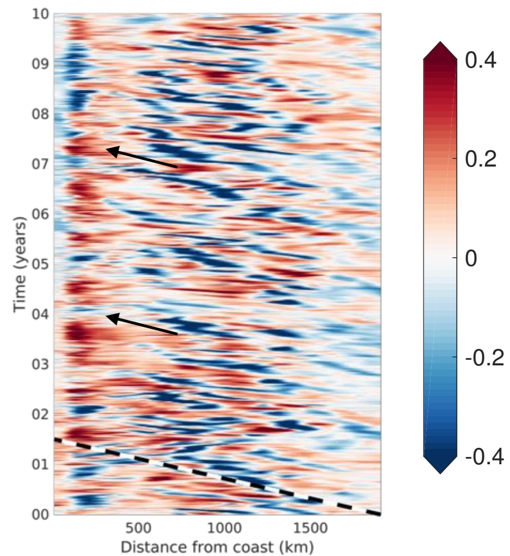
High-resolution
