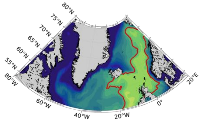
Surface Salinity
