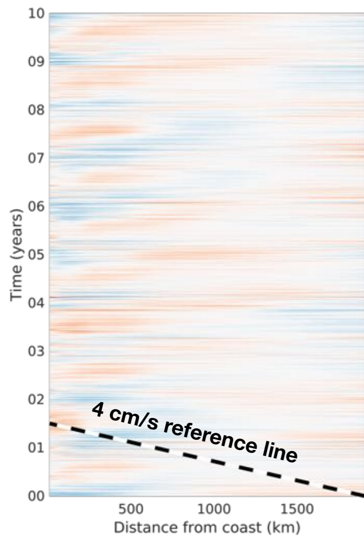
Low-resolution
