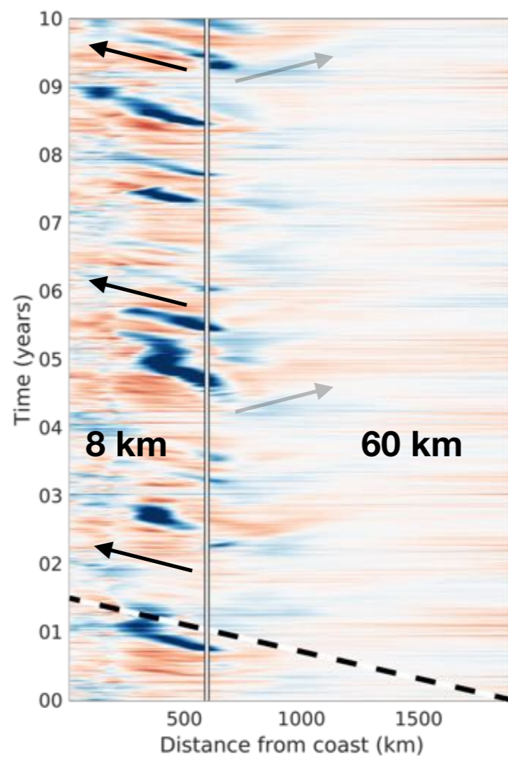
Coastal-refined
