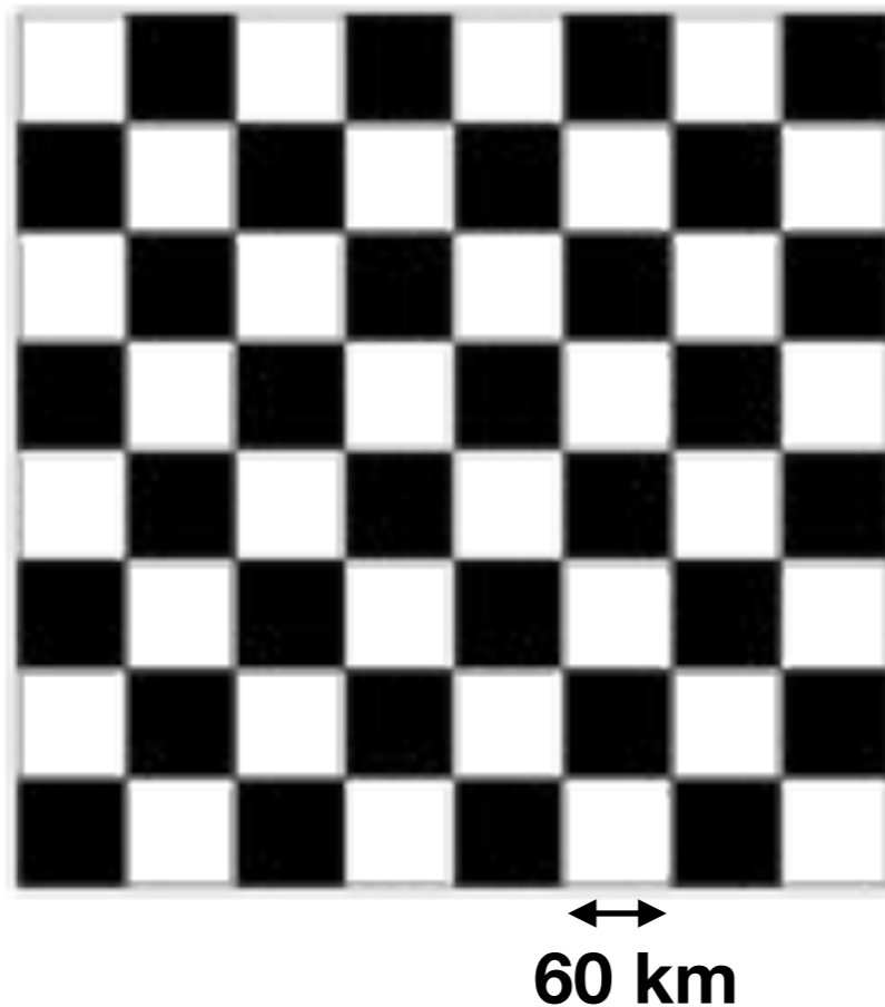
Low-resolution ocean
